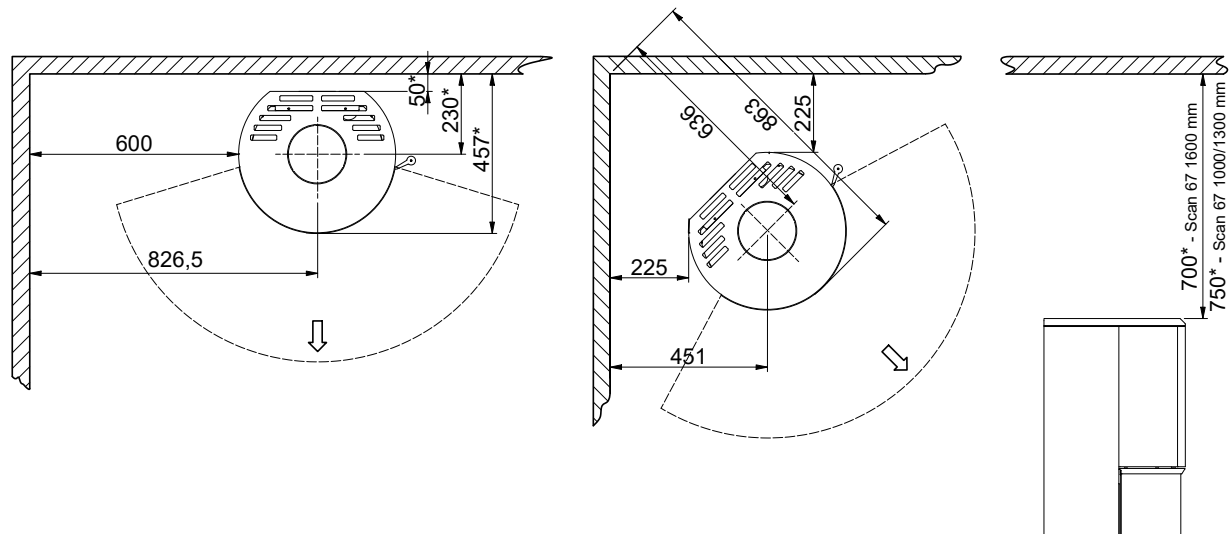
Minimum distance to flammable materials
