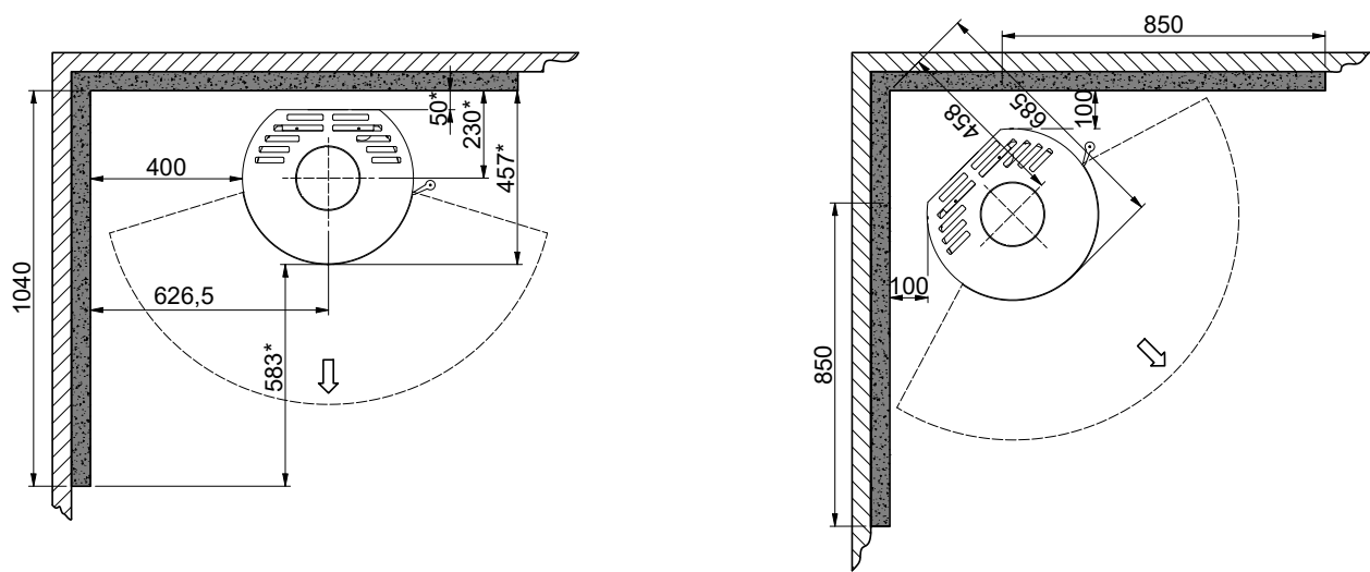
Minimum distance to flammable wall protected by a fire wall
